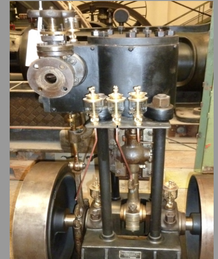
1-Zylinder Dampfmaschine King, Zürich 1920 Losinger, Thun, Technorama
